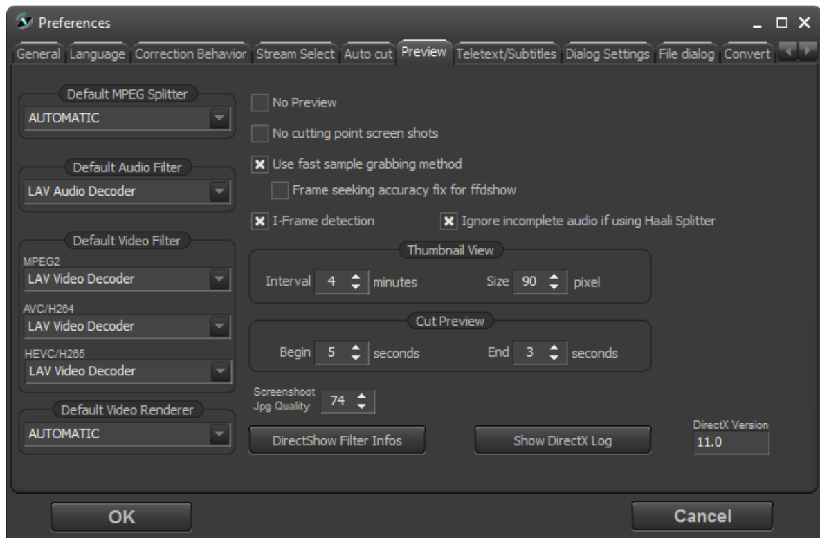
Illustration 3: Manual choice of filters for video preview
